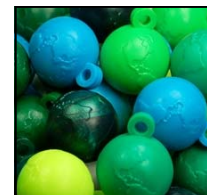
Randoms – globe
